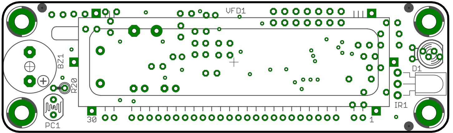
Pict 1. MVFD Panel 16S8D 2.0 top side component layout
