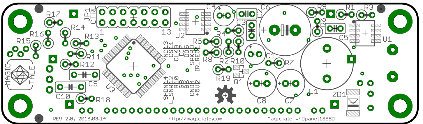
Pict 2. MVFD Panel 16S8D 2.0 bottom side component layout
