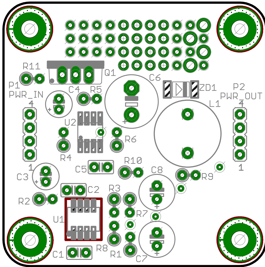
Fig.1. VFD PSU EXP01 top side component layout
