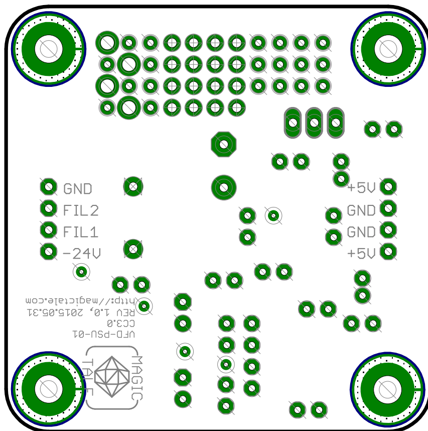
Fig.2. VFD PSU EXP01 bottom side component layout
