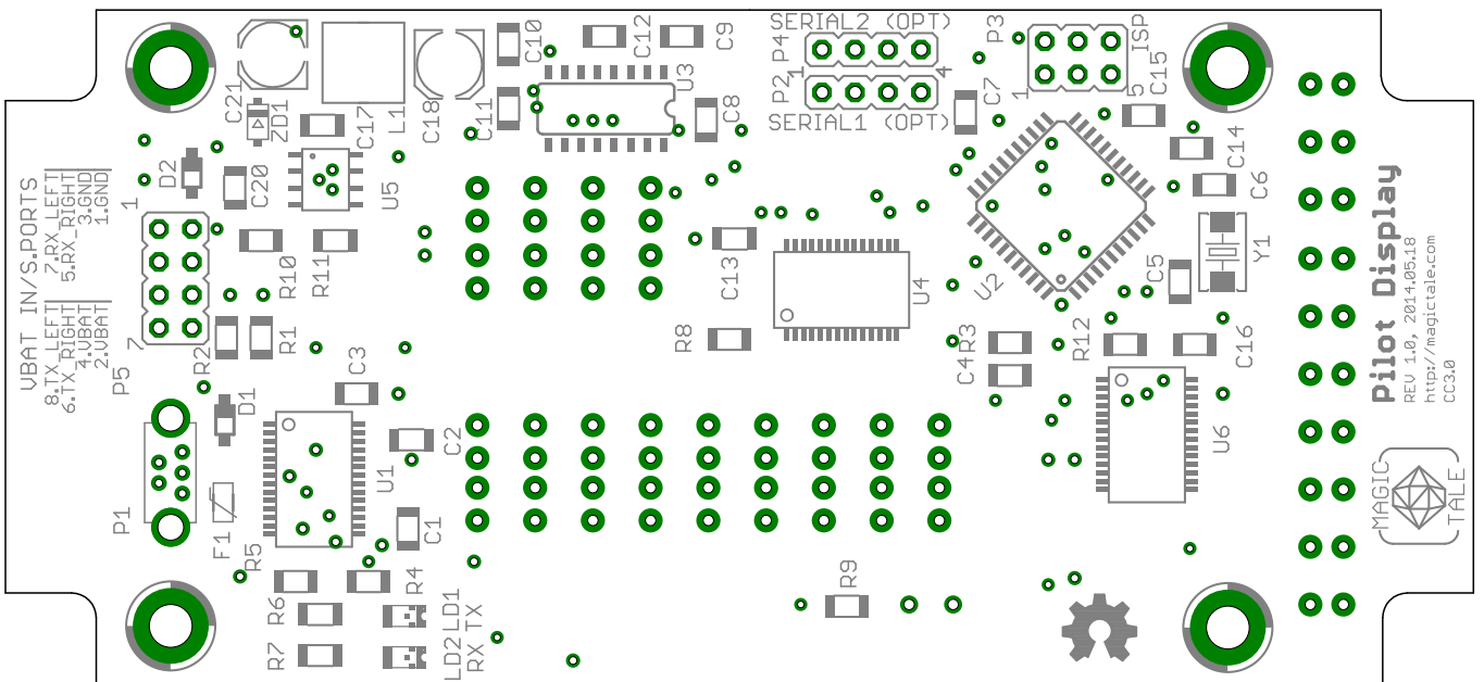
Fig 2. Pilot Display bottom side component layout
