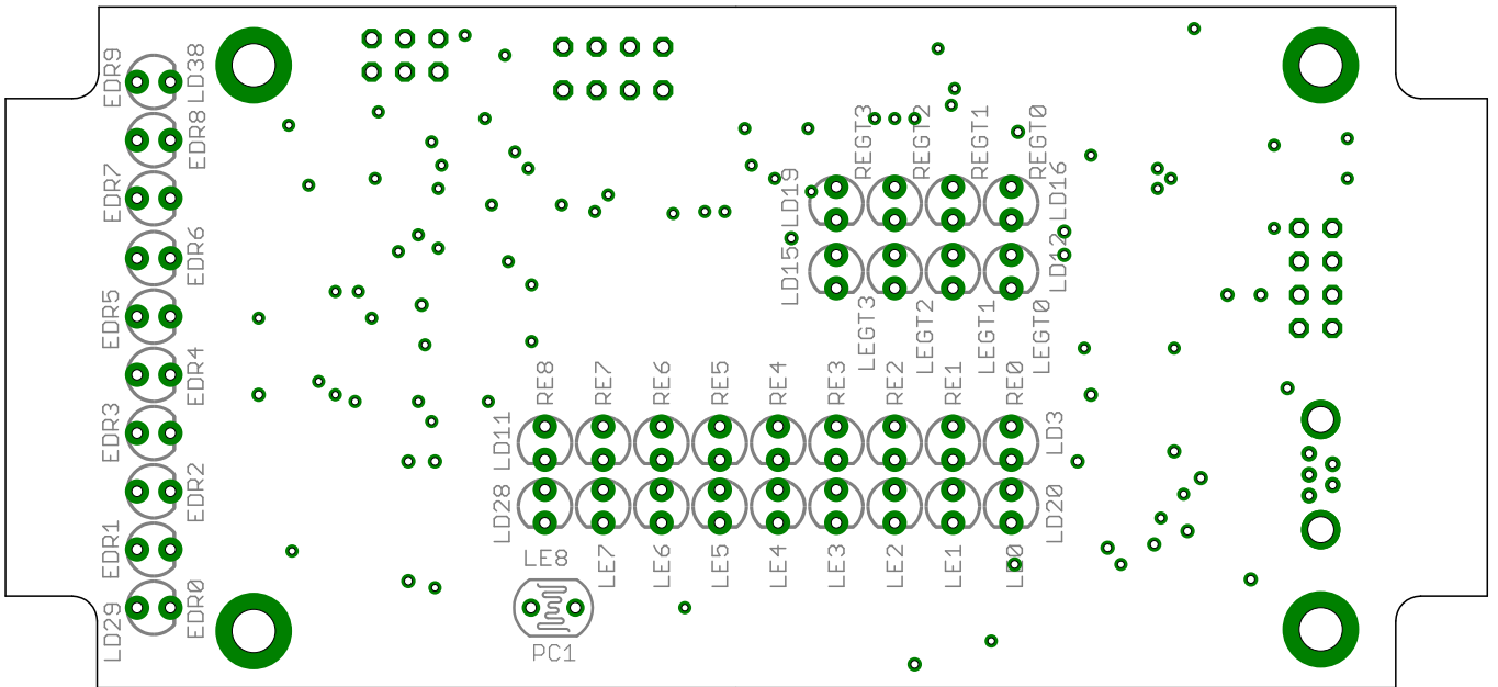
Fig 1. Pilot Display top side component layout
